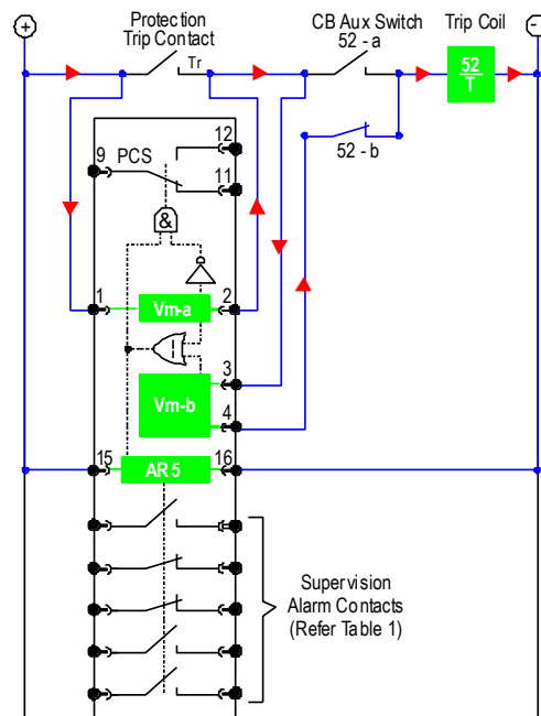
Figure 7: Alpha XR5-00-6 – CB open
