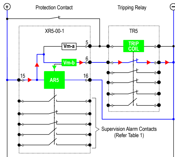
Figure 3: Alpha XR5-00-1 - Tripped condition
