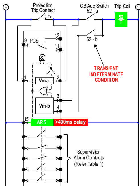
Figure 8: Alpha XR5-00-6 - CB closing
