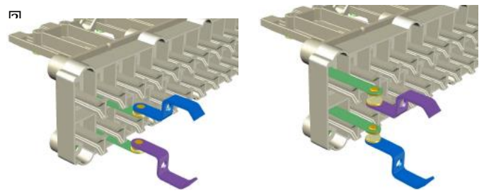
Figure 13: Contact geometry
