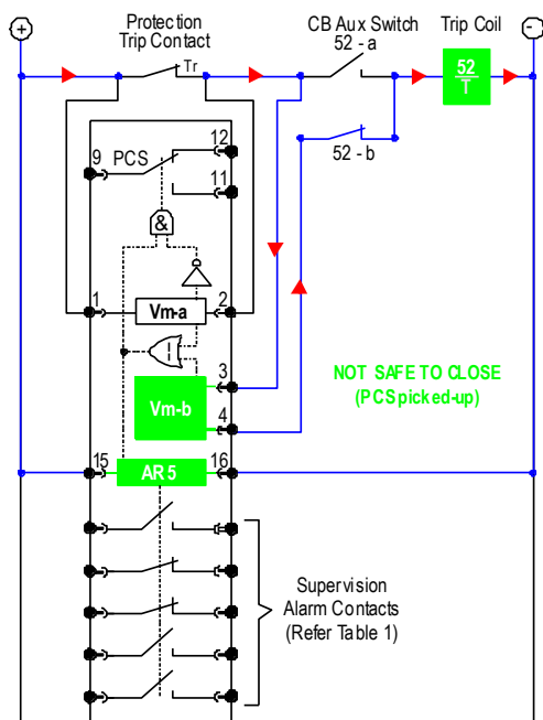
Figure 11: Alpha XR5-00-6 – Tr Closed and CB open
