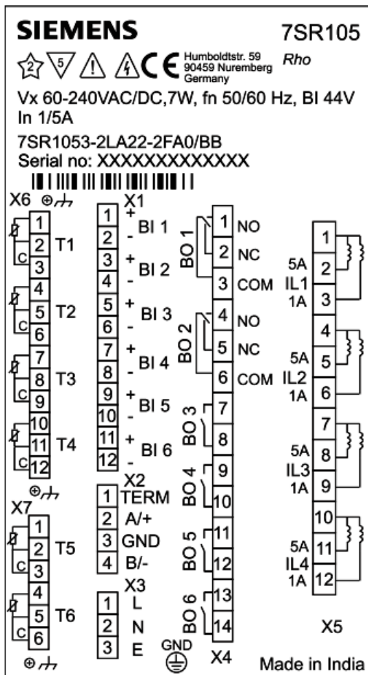
Fig 9. Terminal/Wiring Diagram View (RTD)
