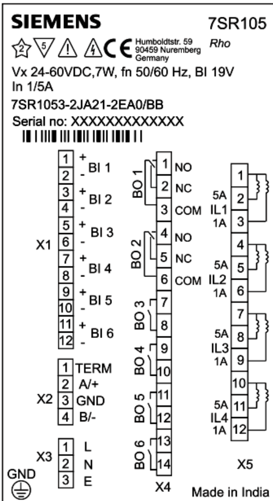
Fig 8. Terminal/Wiring Diagram View (Non RTD)
